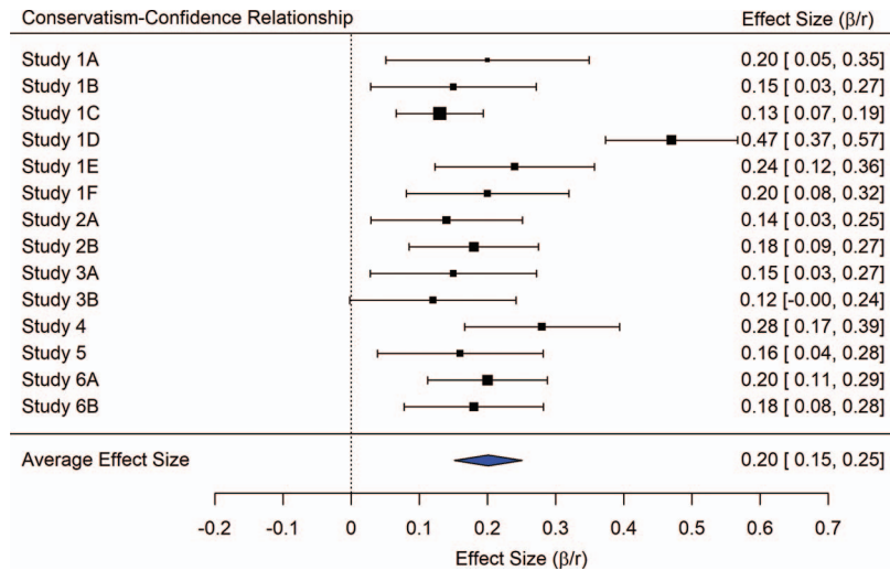
Figure 5. Forest plot of effect sizes of conservatism–confidence relationship, Studies 1A–6B. Average effect size ( \beta/r ) based on a random-effects meta-analysis model. See the online article for the color version of this figure.
